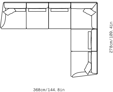
Comp. 06 (MDB2+MD1+RI+MP1+MDB2)
