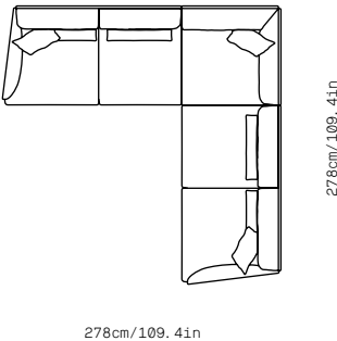
Comp. 05 (MDB2+MD1+RI+MD2+MP1)
